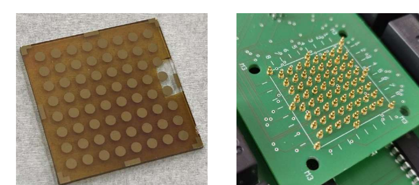
Fig. 4 A device design and measurement setup for combinatorial photovoltaic analysis are currently under development. It will allow to characterize 64 cells in a single run.
