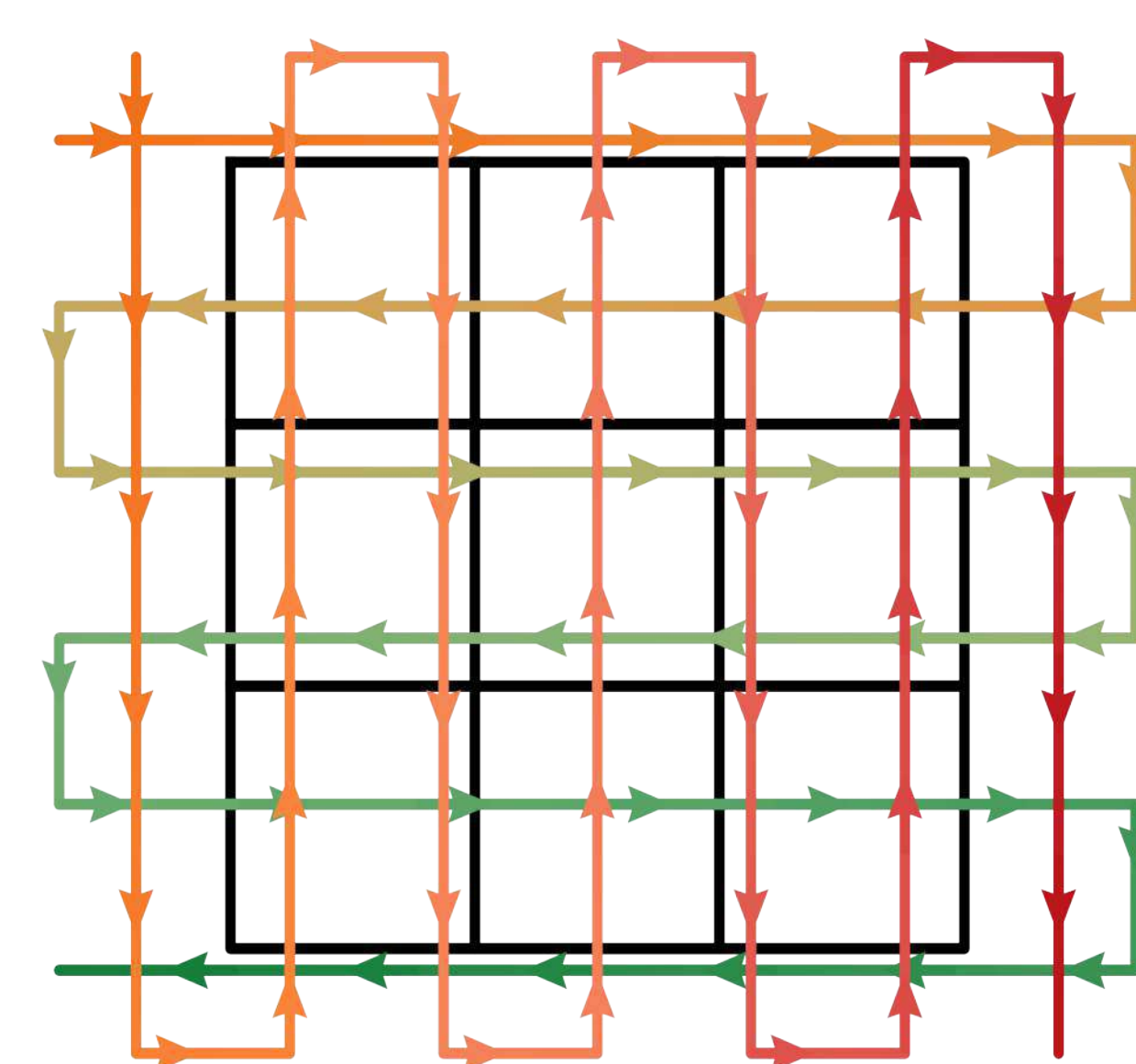
Fig. 6 Combinatorial spray pattern which alternates between a vertical Cu-Ga gradient (orange to green) and a horizontal Cu-Fe gradient (orange to red). The number of displayed scan lines is reduced from 25 and 27, resp., in order to simplify the illustration.
