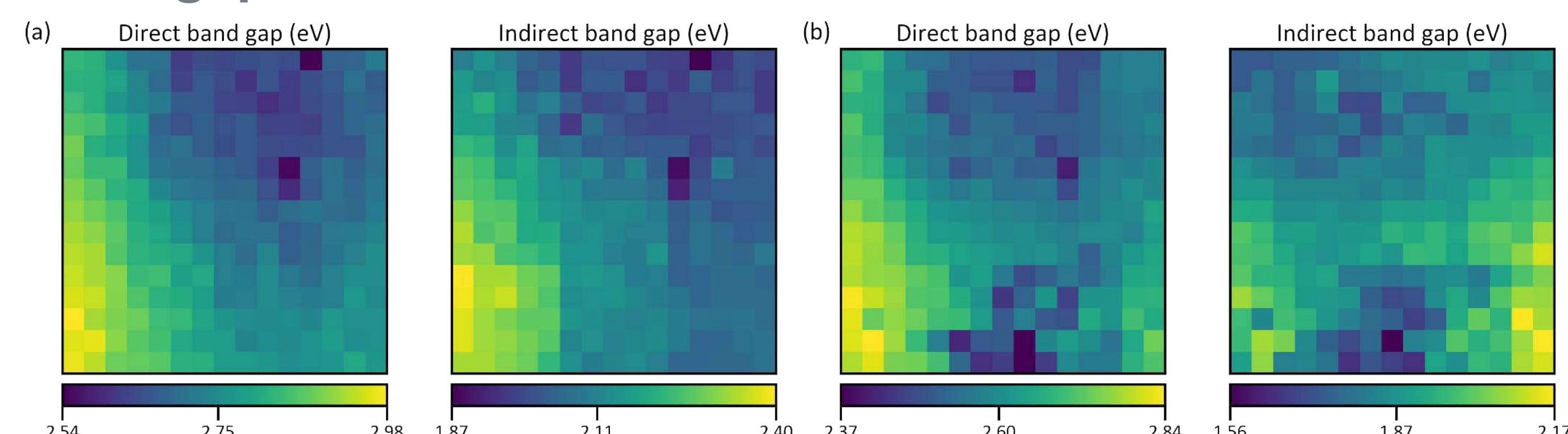
Fig. 4 Maps of direct and indirect band gaps evaluated using the Tauc method (a) for the as-deposited film, and (b) for the same film after annealing at 550 °C for 2 h under N 2 . The values of the colour bars are the minimum, the mean, and the maximum band gap energy.
